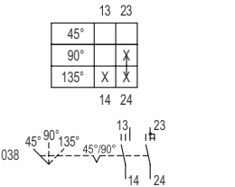
Switching arrangement 8008/-038
