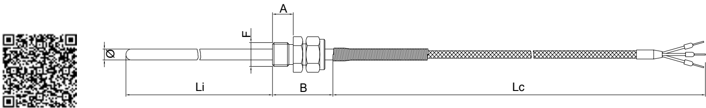
TR1 B: with sliding pressure mount
