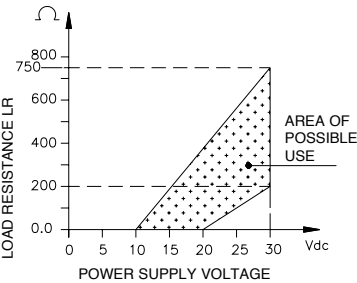
LOAD DIAGRAM (Output current)
